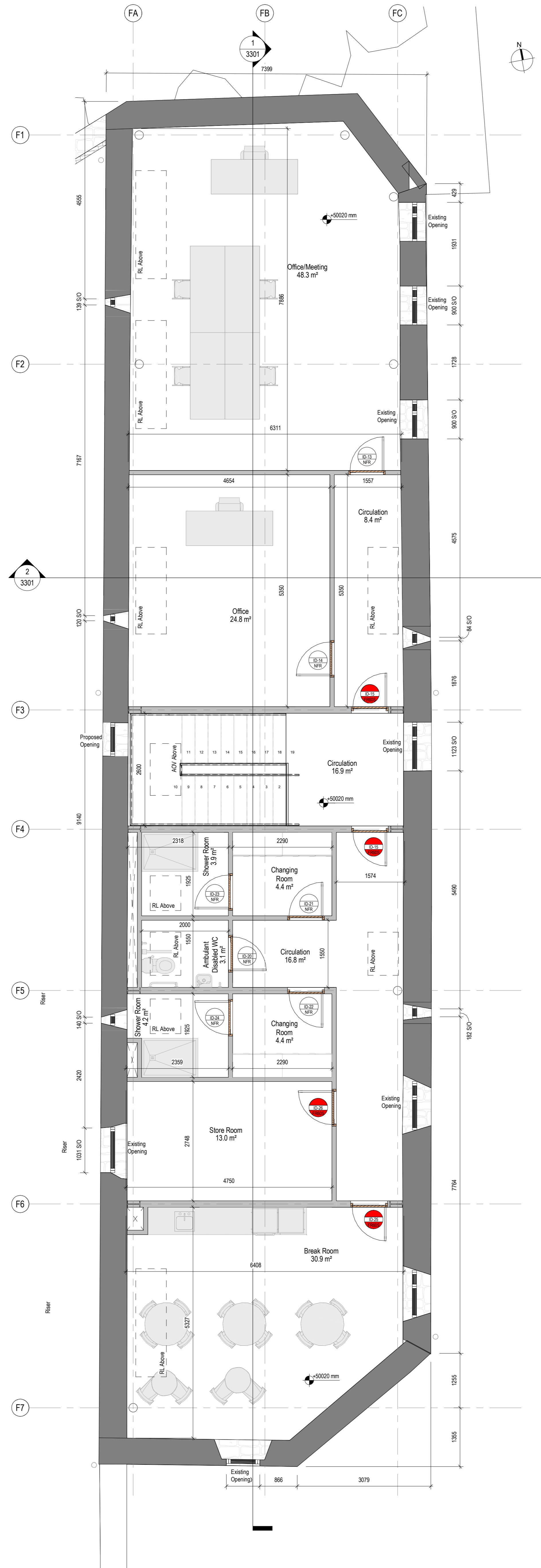
2 FL1 Proposed First Floor 2302 Scale: 1:50
